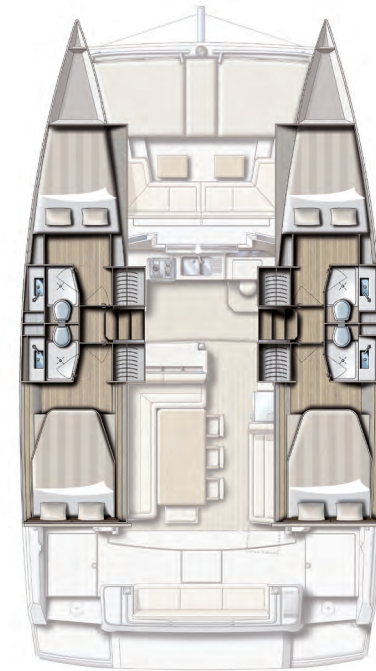
Version 4 cabines / 4 sdb 4 cabins and 4 baths version
